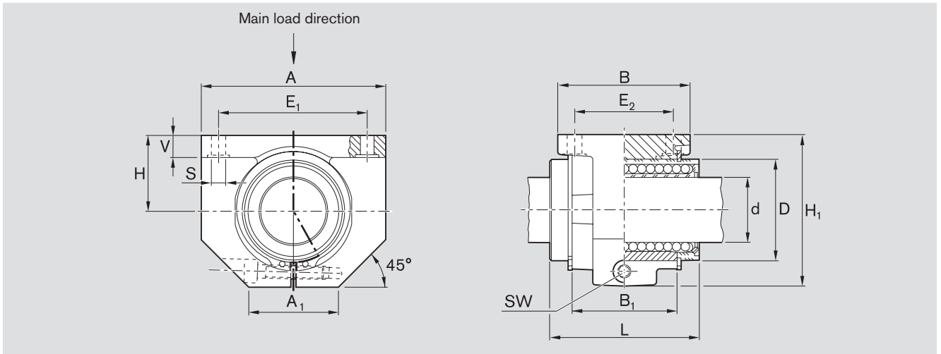
Dimensions (mm)
